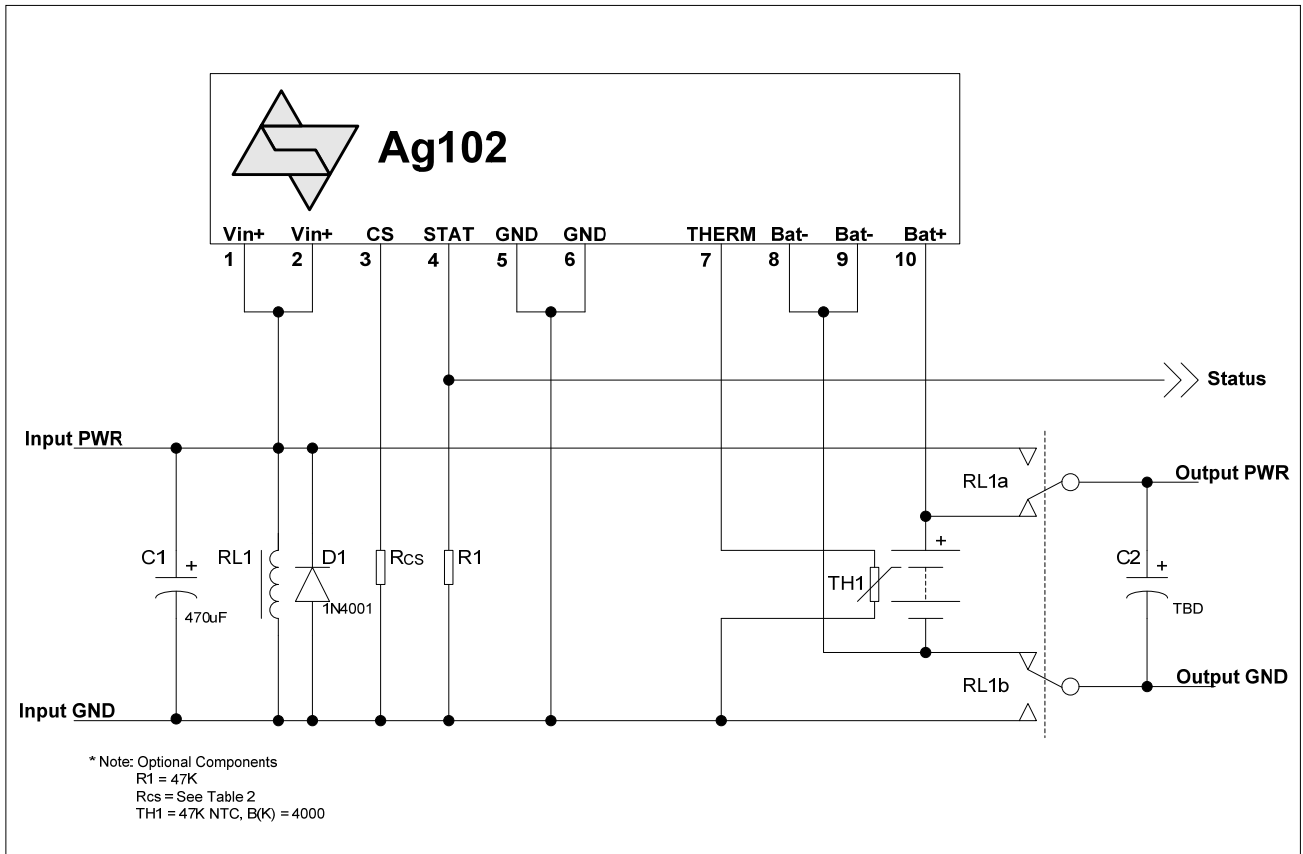
Figure 9: Typical Application
