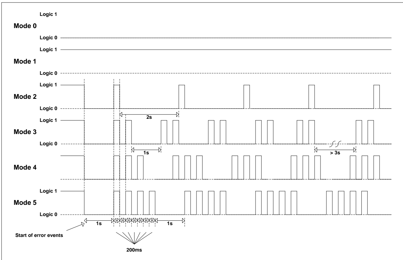
Figure 8: STAT Output Timing
