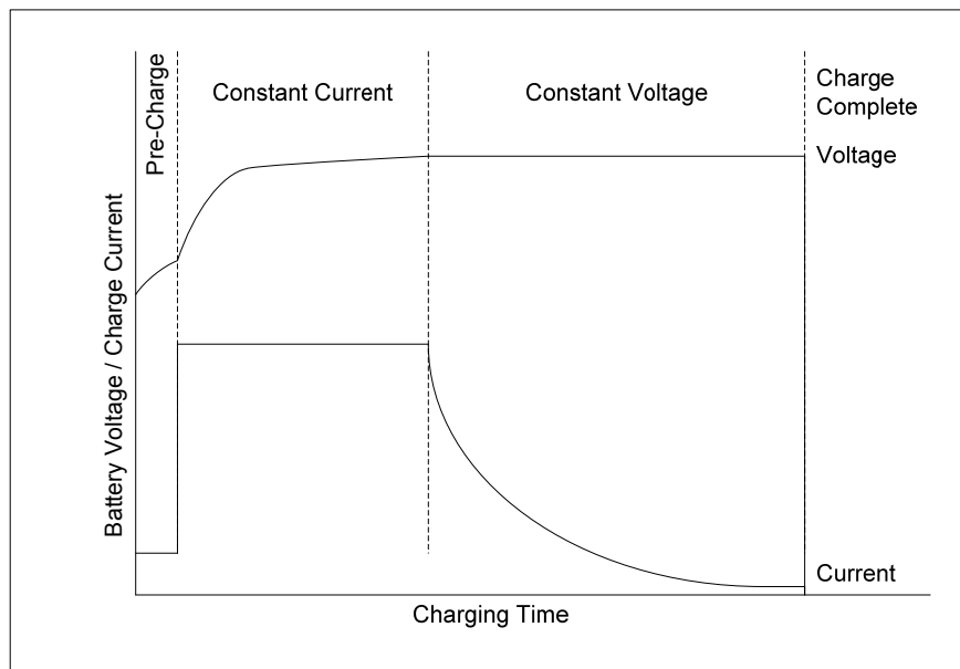
Figure 3: Basic Ag112 Charge Profile
